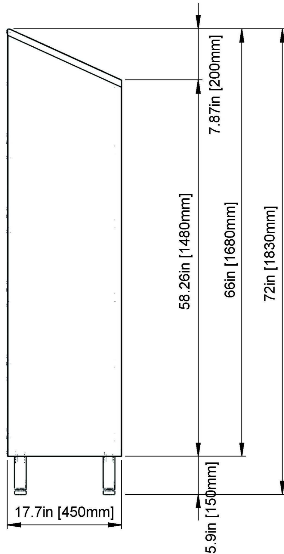
Full assembly
